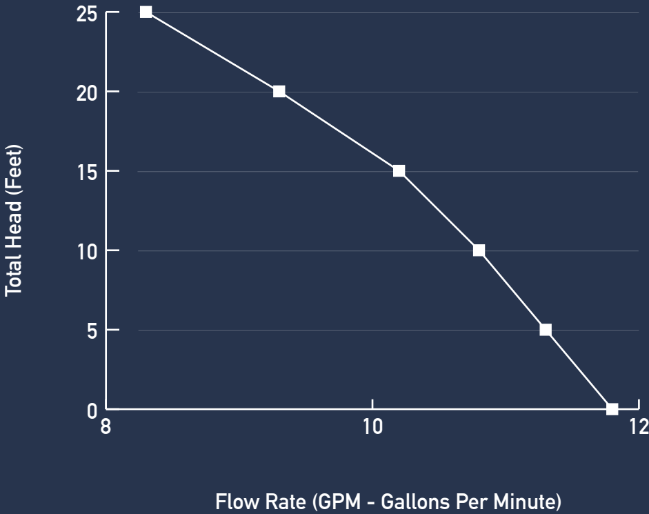
Approximate gallons per minute output at 40 psi (Maximum pressure 74 psi)
