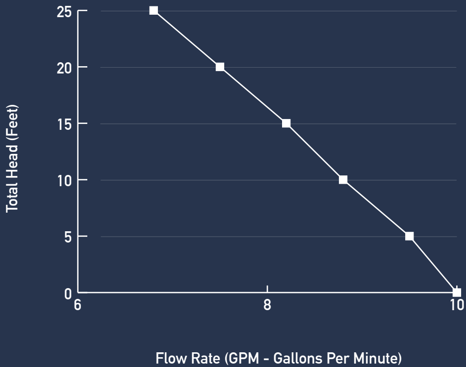
Approximate gallons per minute output at 40 psi (Maximum pressure 67 psi)
