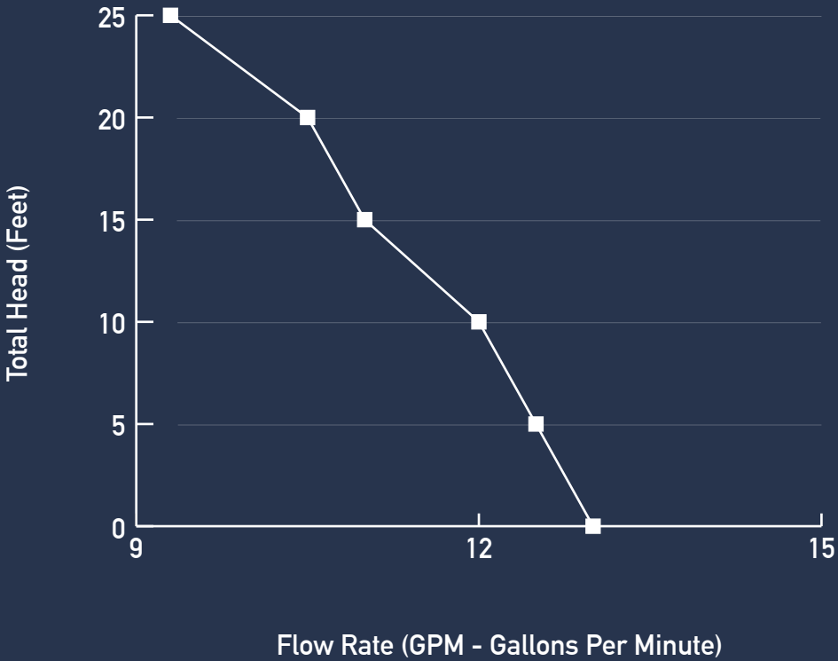
Approximate gallons per minute output at 40 psi (Maximum pressure 79 psi)
